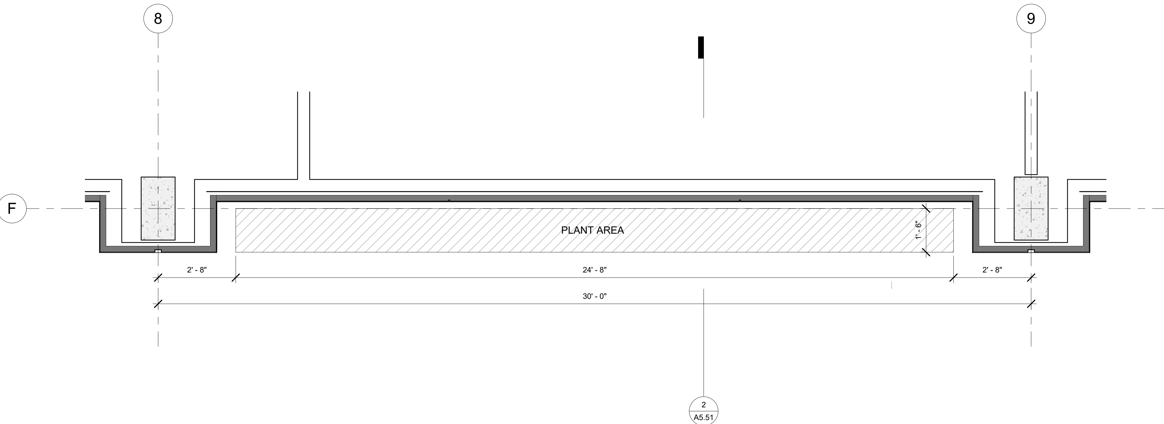
3 PLAN 1/2" = 1'-0"
