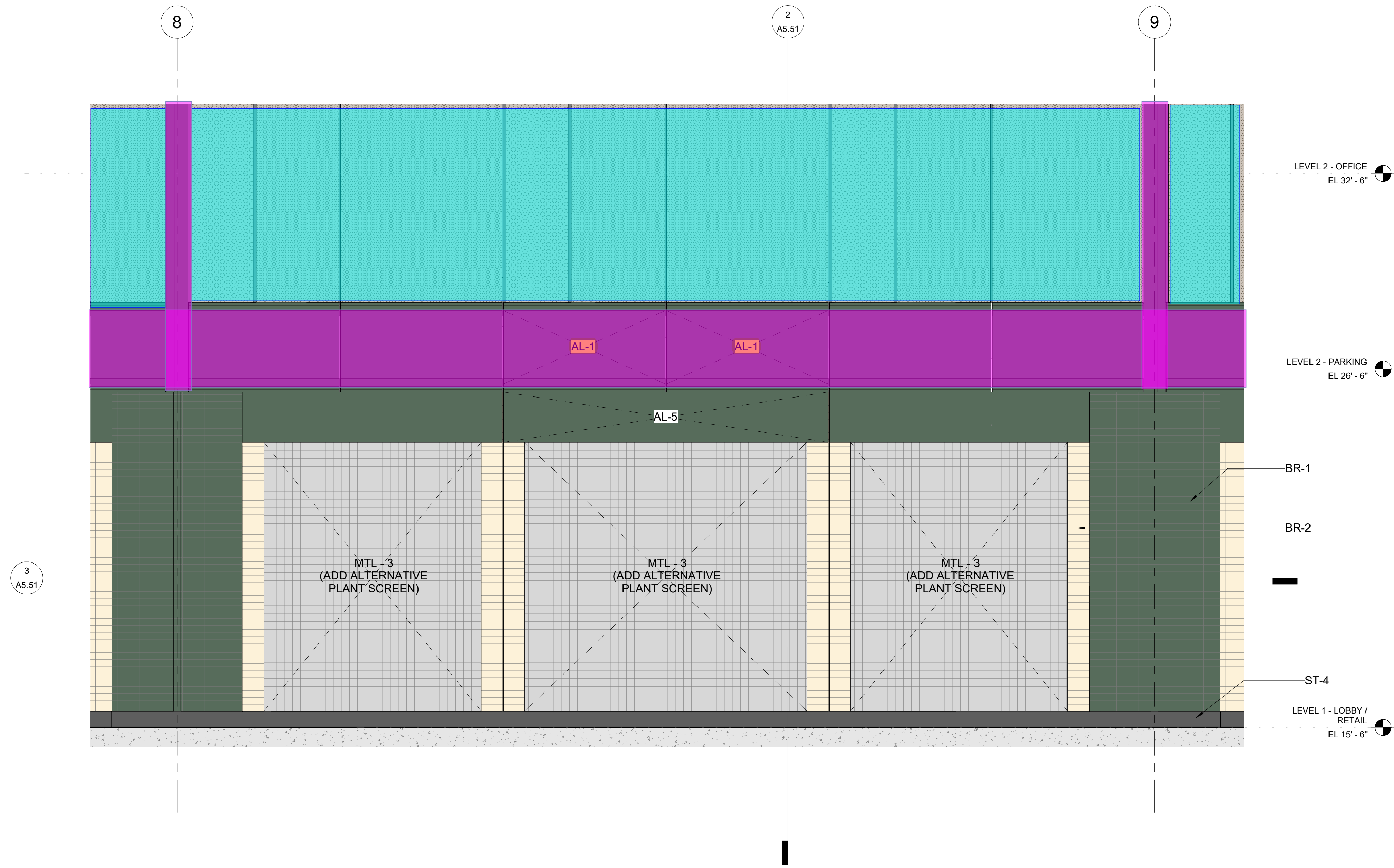
1 ELEVATION 1/2" = 1'-0"
